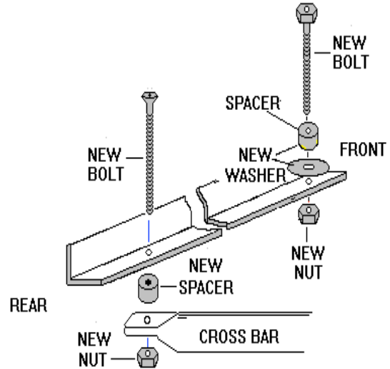
NEW SET-UP FOR SUPPORT BRACKET
